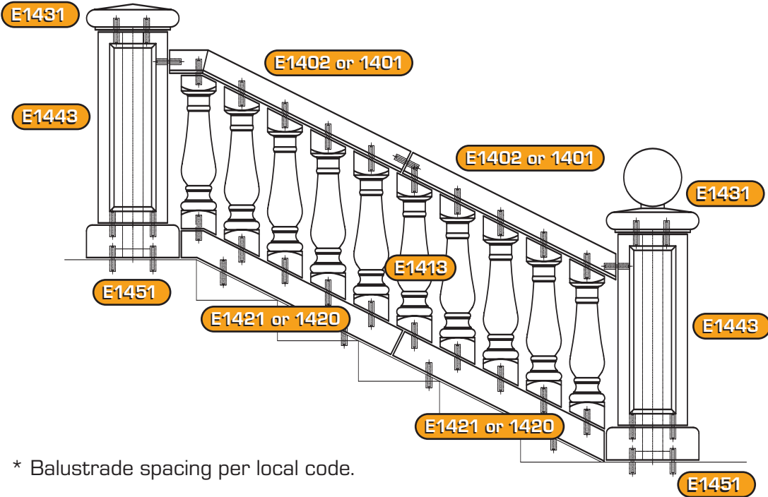
Elevation view of rail system at stairs.
