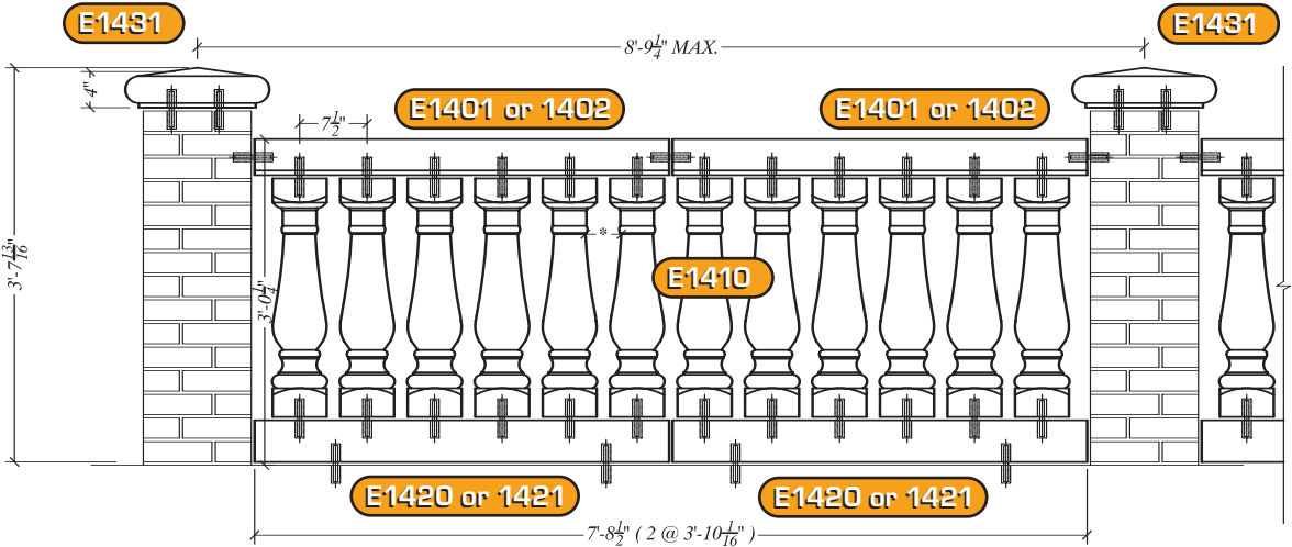
Elevation view of rail system with brick piers.
